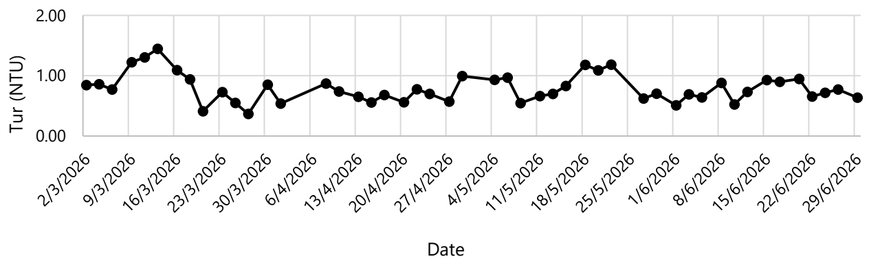
Turbidity (Flood)
